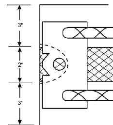
8" SANDWICH PANEL (3" X 2" X 3")
